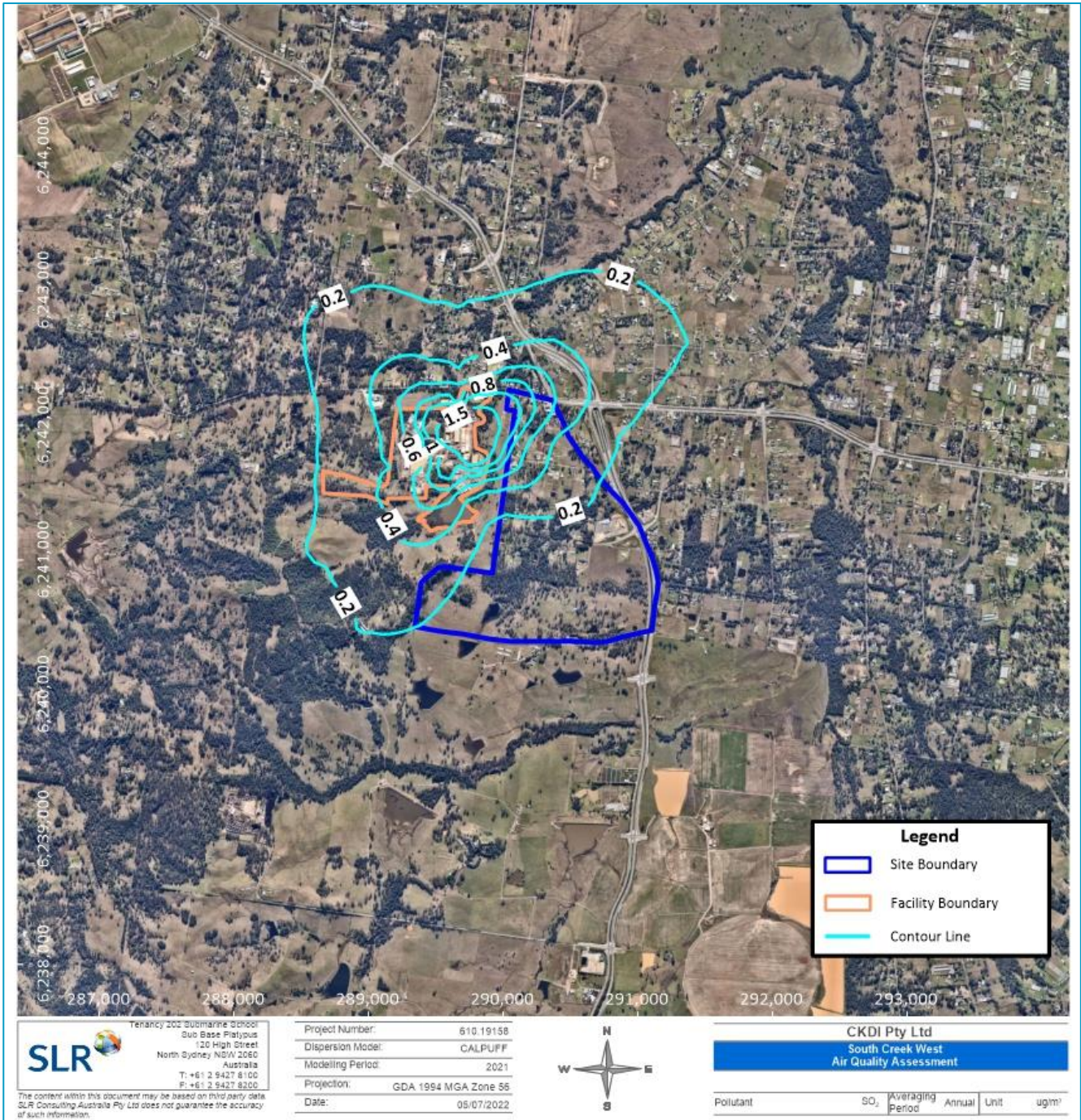
Figure D-15 Predicted Annual Average Incremental SO 2 Isoleth Plot
