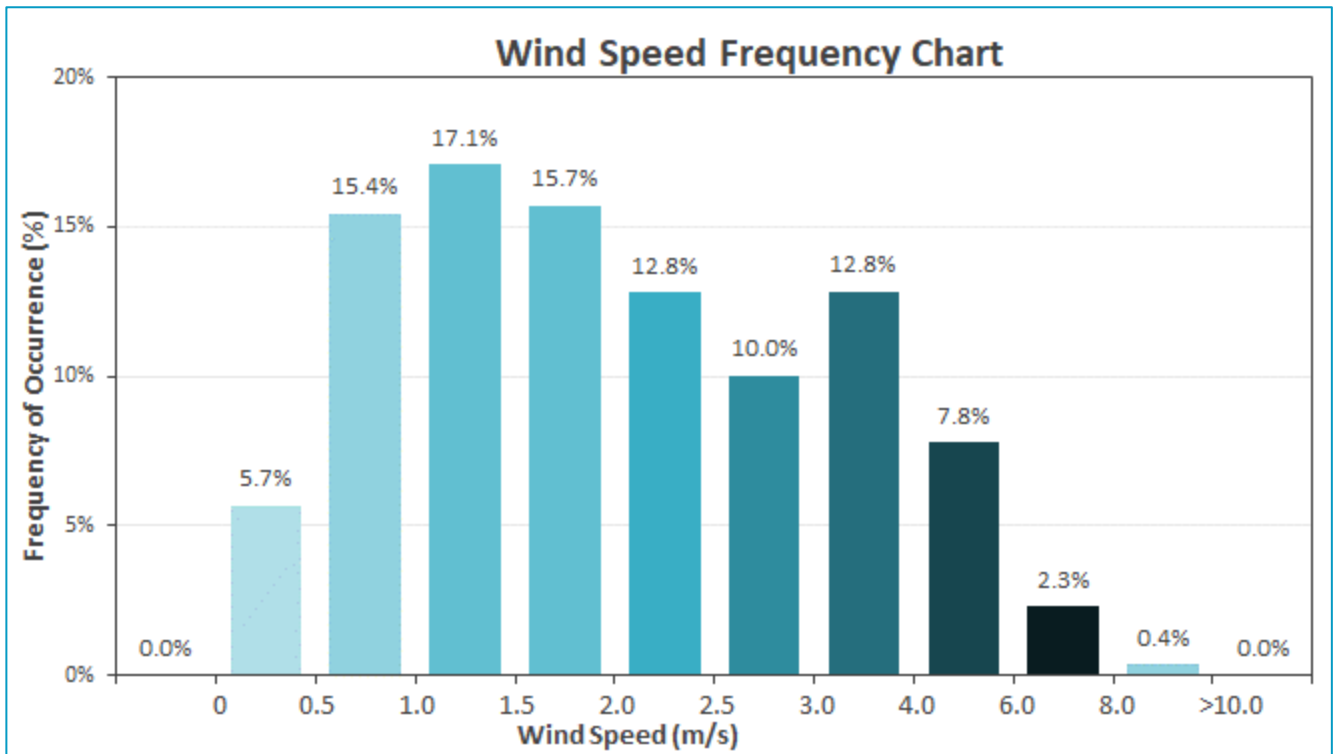
Figure 16 Annual Wind Speed Frequencies at the Site (CALMET Predictions, 2021)
