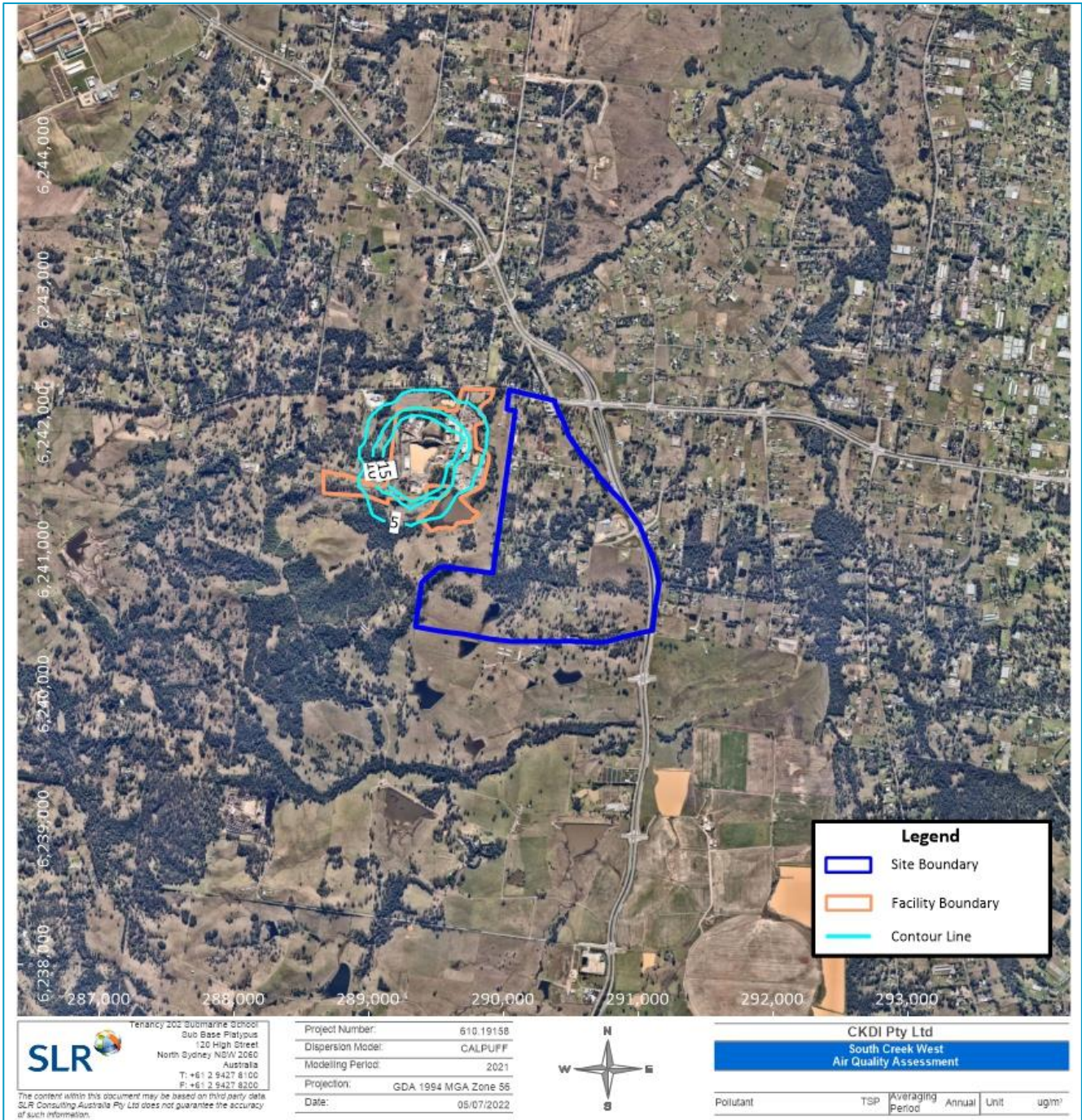
Figure B-3 Predicted Annual Average Incremental TSP Isoleth Plot
