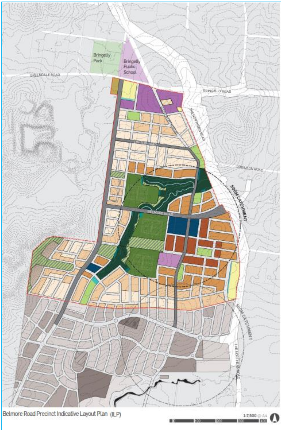
Figure 2 Indicative Site Layout – Precinct 2
