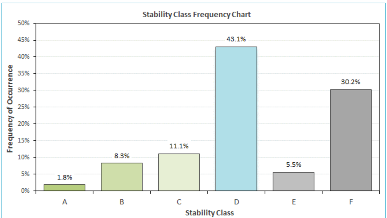
Figure 17 Predicted Stability Class Frequencies at the Site (CALMET predictions, 2021)
