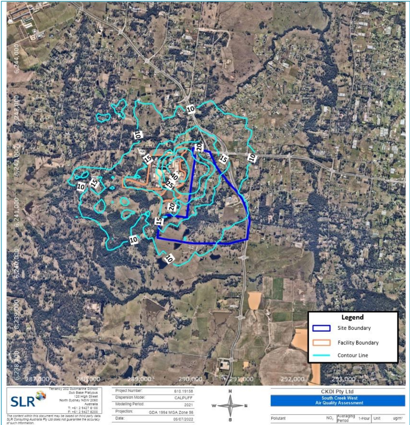
Figure B-10 Predicted 1-Hour Average Incremental NO 2 Isoleth Plot
