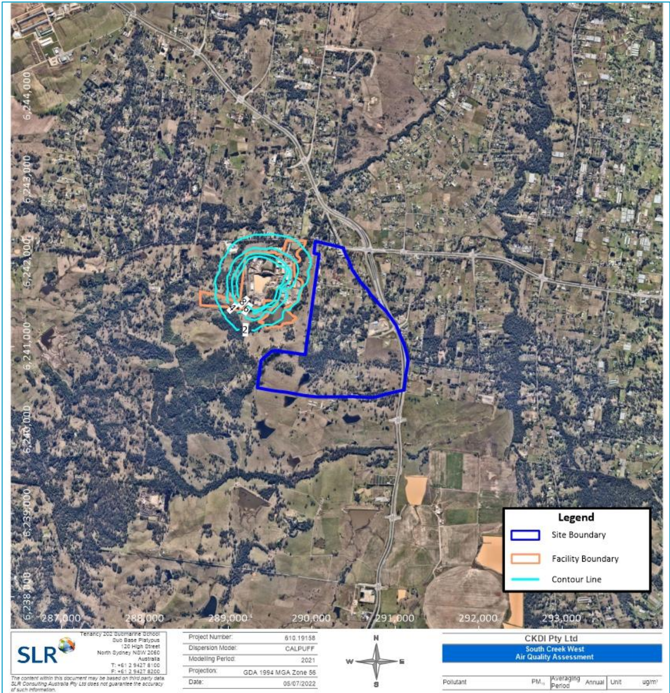
Figure B-2 Predicted Annual Average Incremental PM 10 Isoleth Plot
