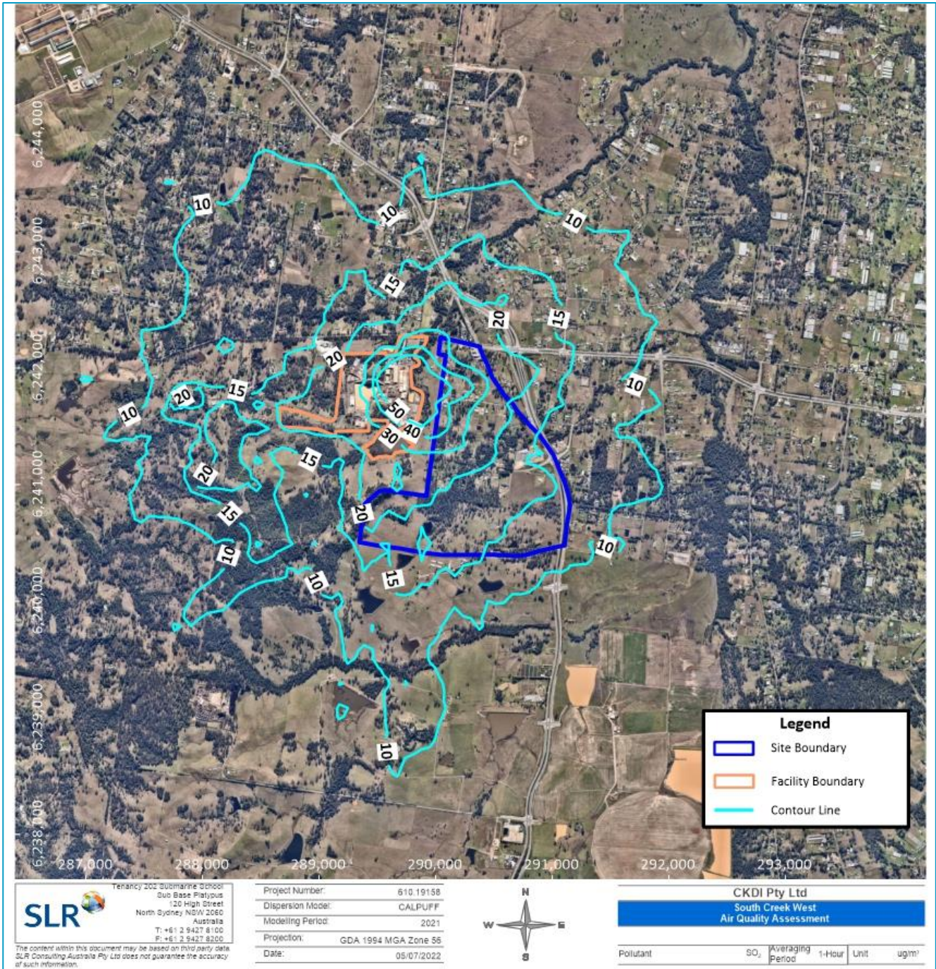
Figure D-13 Predicted 1-Hour Average Incremental SO 2 Isoleth Plot
